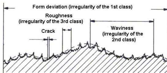
Fig. 1. Types of surface irregularities [1].
