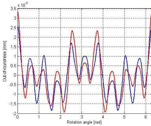
Fig. 2. Plots of compared roundness profiles in Cartesian coordinates.
