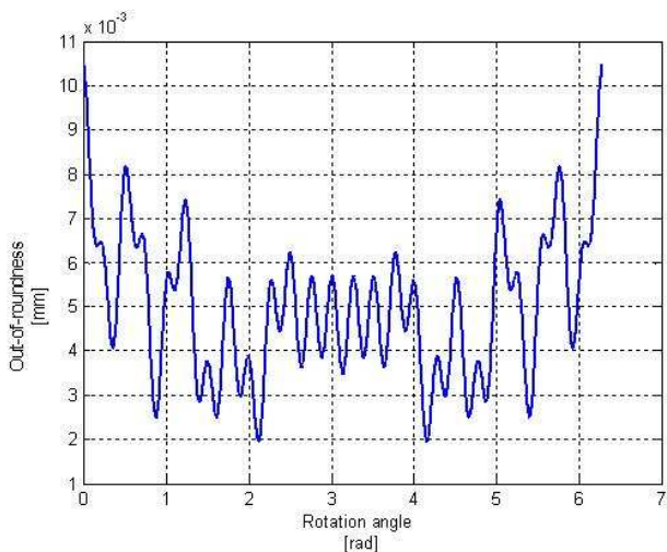
Fig. 7. The roundness profile given by formula (10).
